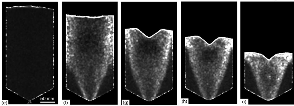
Figure 2. Radiograph sequence of silo discharging in the case of loose packing and smooth silo wall. Rescaled radiographs for (a) initial packing ( t_n=0 ) and (b) after t_n=0.04 of discharging process. (c) subtraction (b) and its previous frame and (d) corresponding variance map, together with a scale bar. (e-i) sequence of variance maps @ t_n=0, t_n=0.04, t_n=0.2, t_n=0.28 and t_n=0.45 . Same scale bar as in (d).
