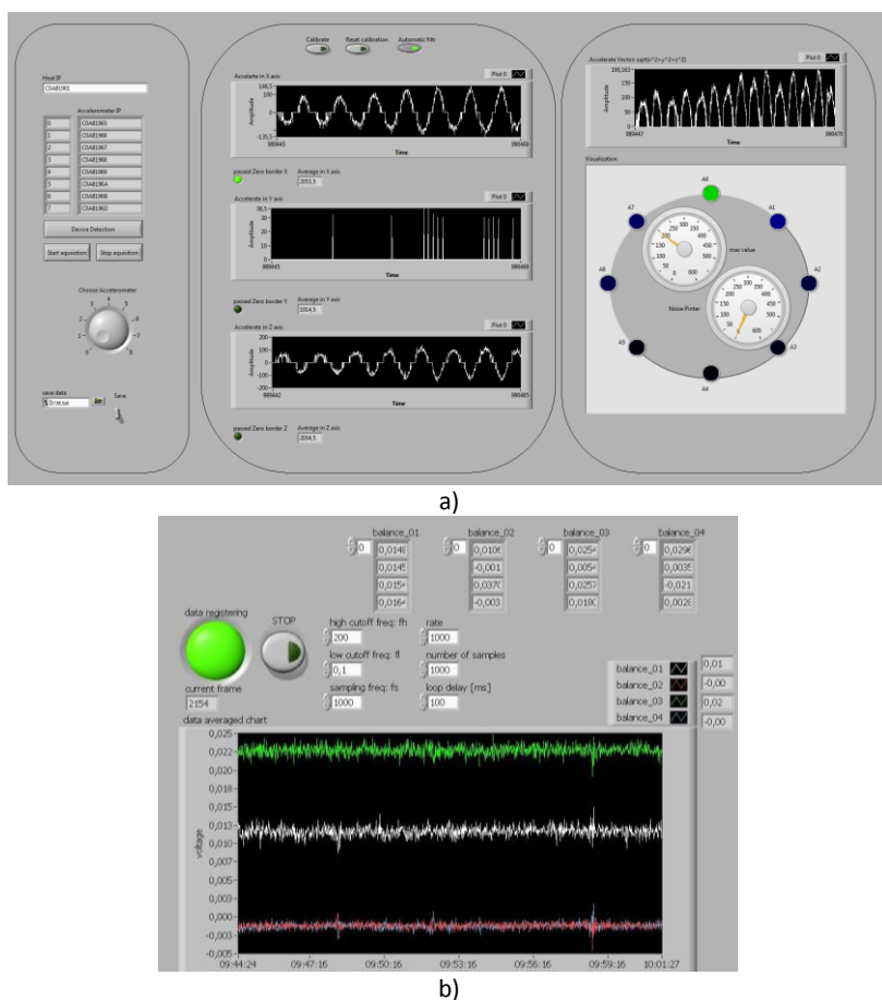
Fig. 4. User interface control and monitoring PC screen a) accelerometer modul, b) tensometer modul
