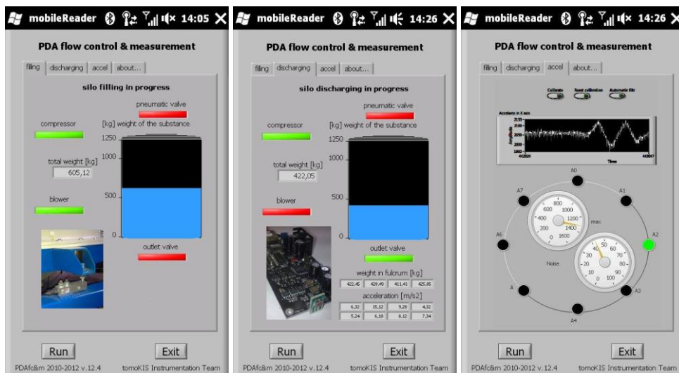
Fig. 5. User interface control and monitoring PDA screens
