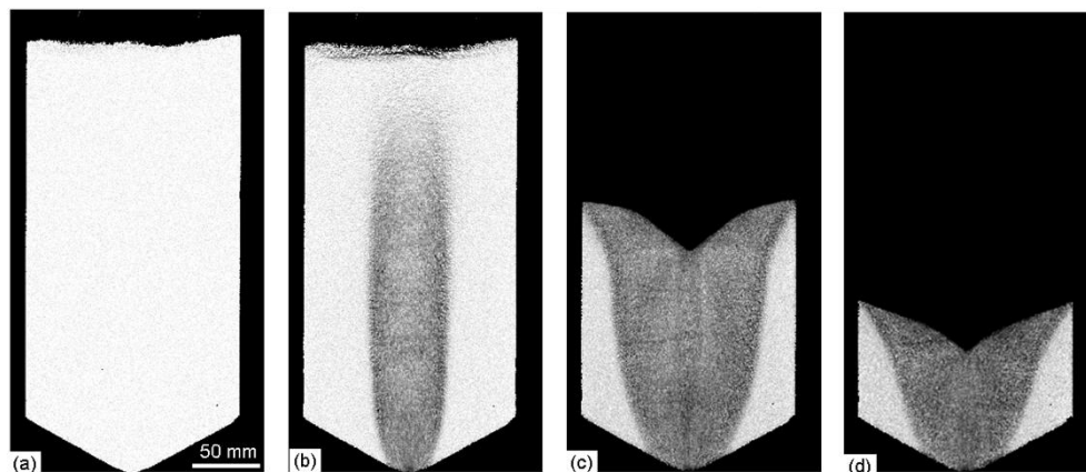
Figure 1. Normalised radiograph sequence showing silo discharging in the case of dense packing and smooth silo walls. (a-d) sequence at normalised times t_n=0 , t_n=0.04 , t_n=0.5 and t_n=0.75 .
