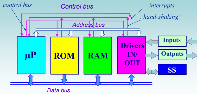
Computer scheme showing its constructive modules
