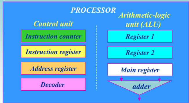
Basic processor modules
