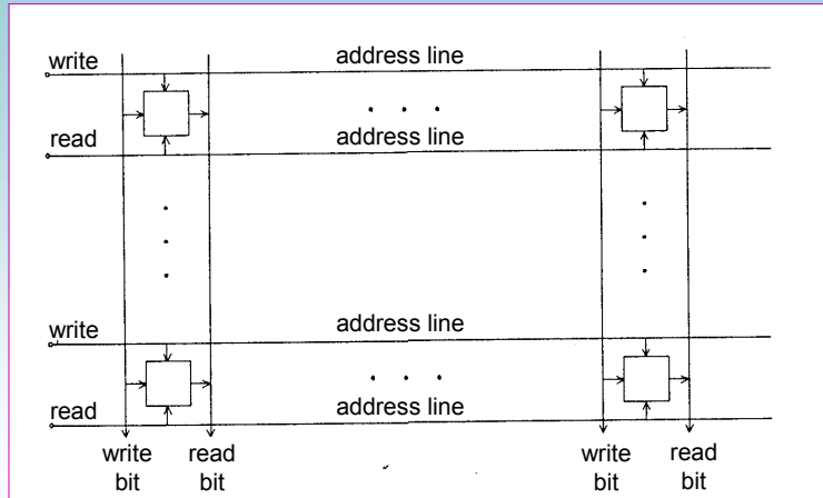
RAM physical structure
