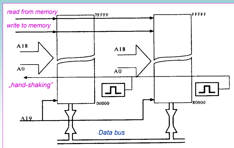
Scheme of RAM block
